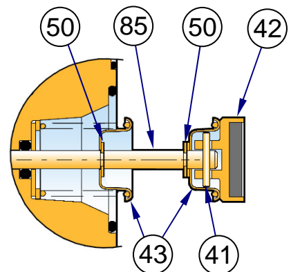
ALTERNATIVE VALVE FOR FLANGED UNITS
