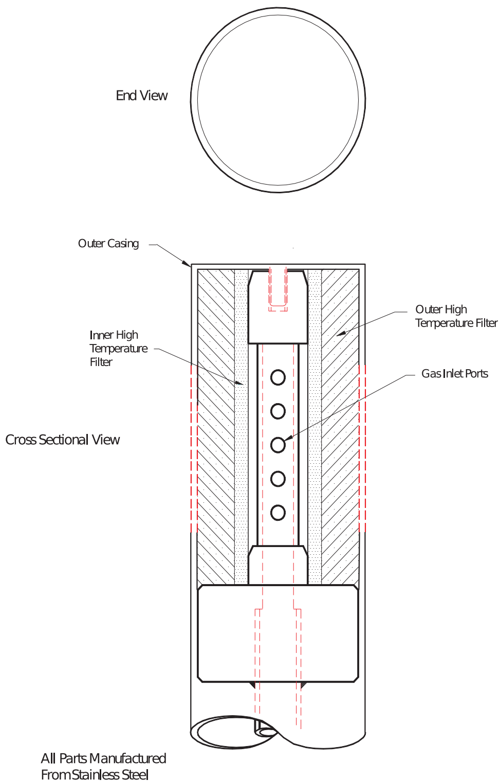
Figure 1.6.2.i Sampling Probe Internal Layout
