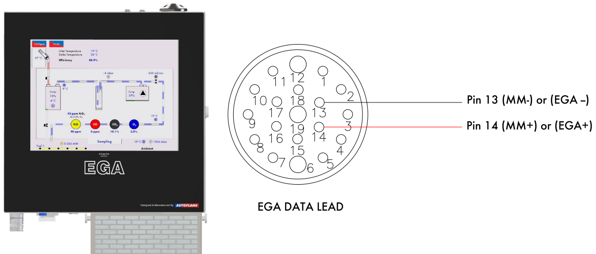
Figure 5.2 Direct Modbus connections on the EGA's flying lead
