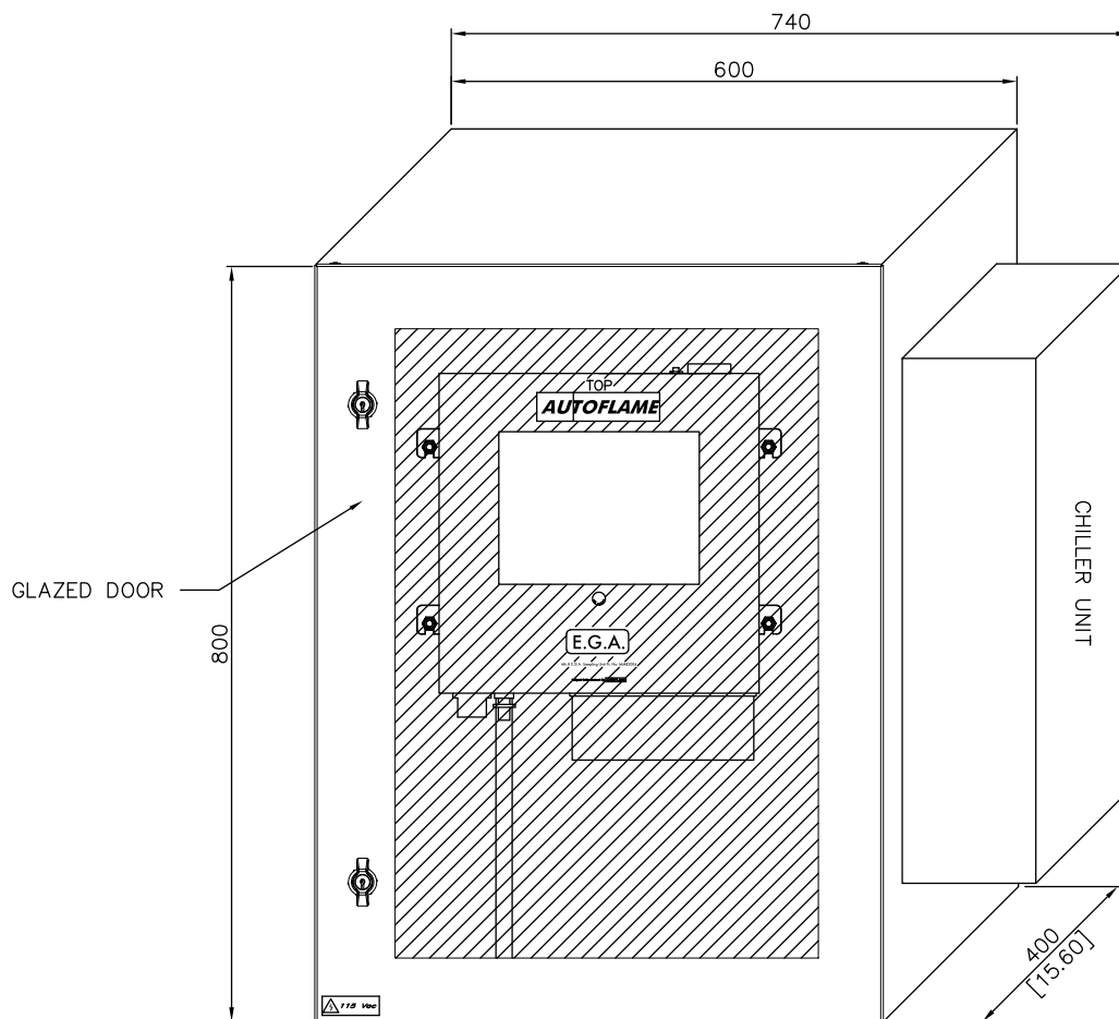
Figure 1.8.3.i Schematic of EGA Chilled Environmental Enclosure
