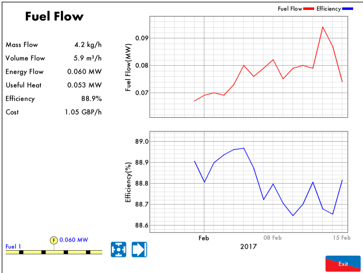
Figure 4.1.4.i Fuel Flow
