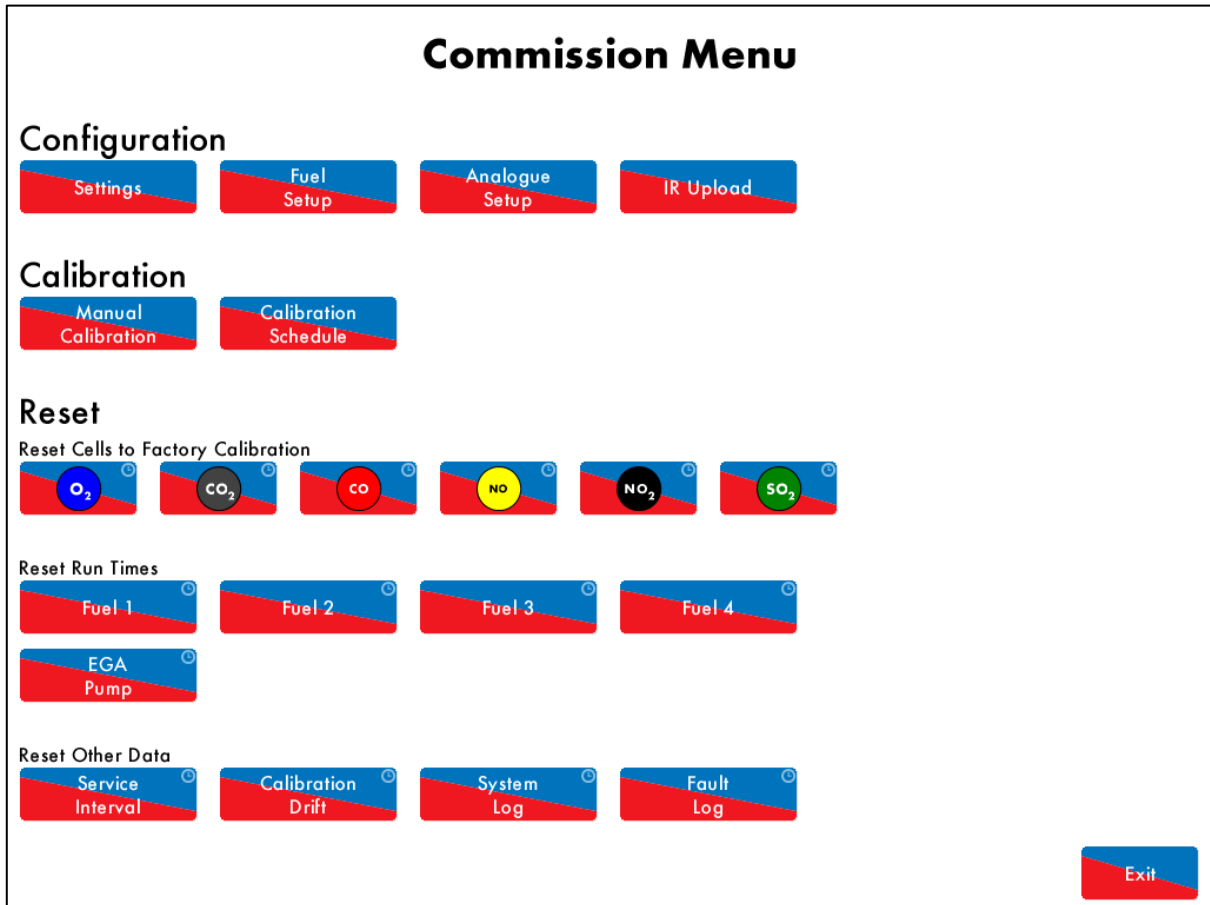
Figure 2.2.iii Commission Menu
