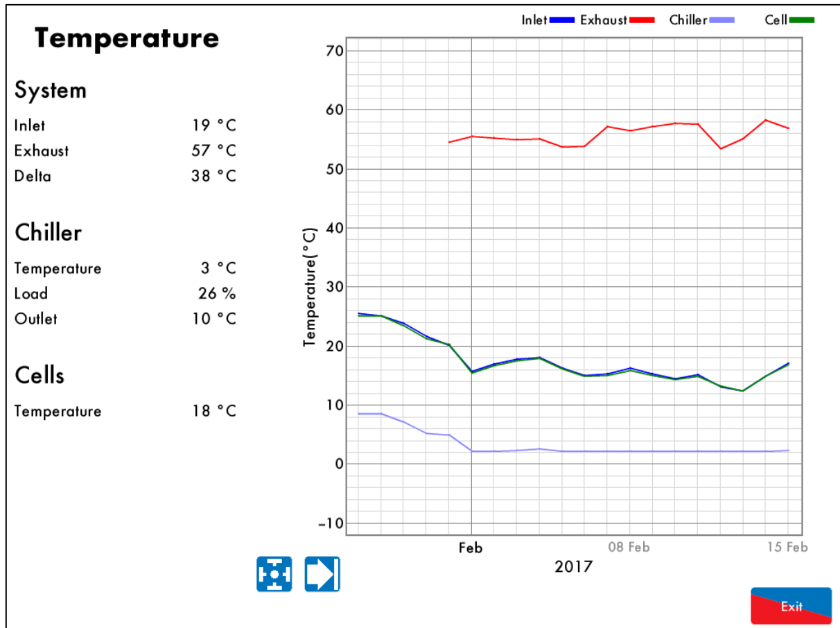
Figure 4.1.1.i Temperature screen on the EGA
