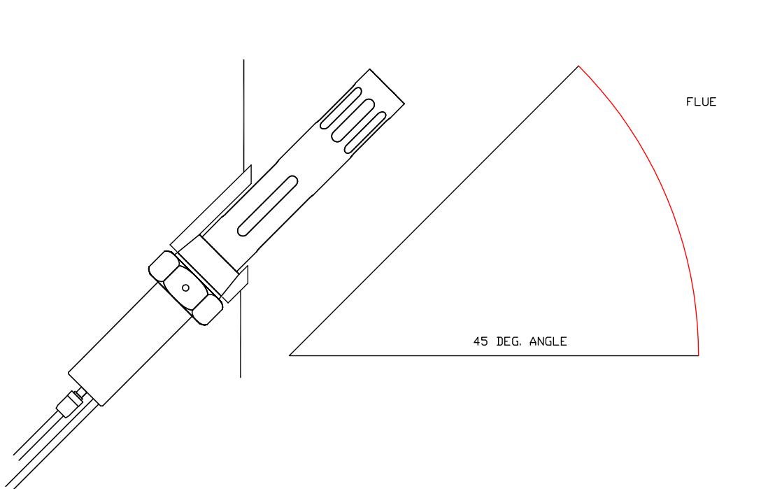
Figure 1.6.4.i EGA Probe 45° In Flue
