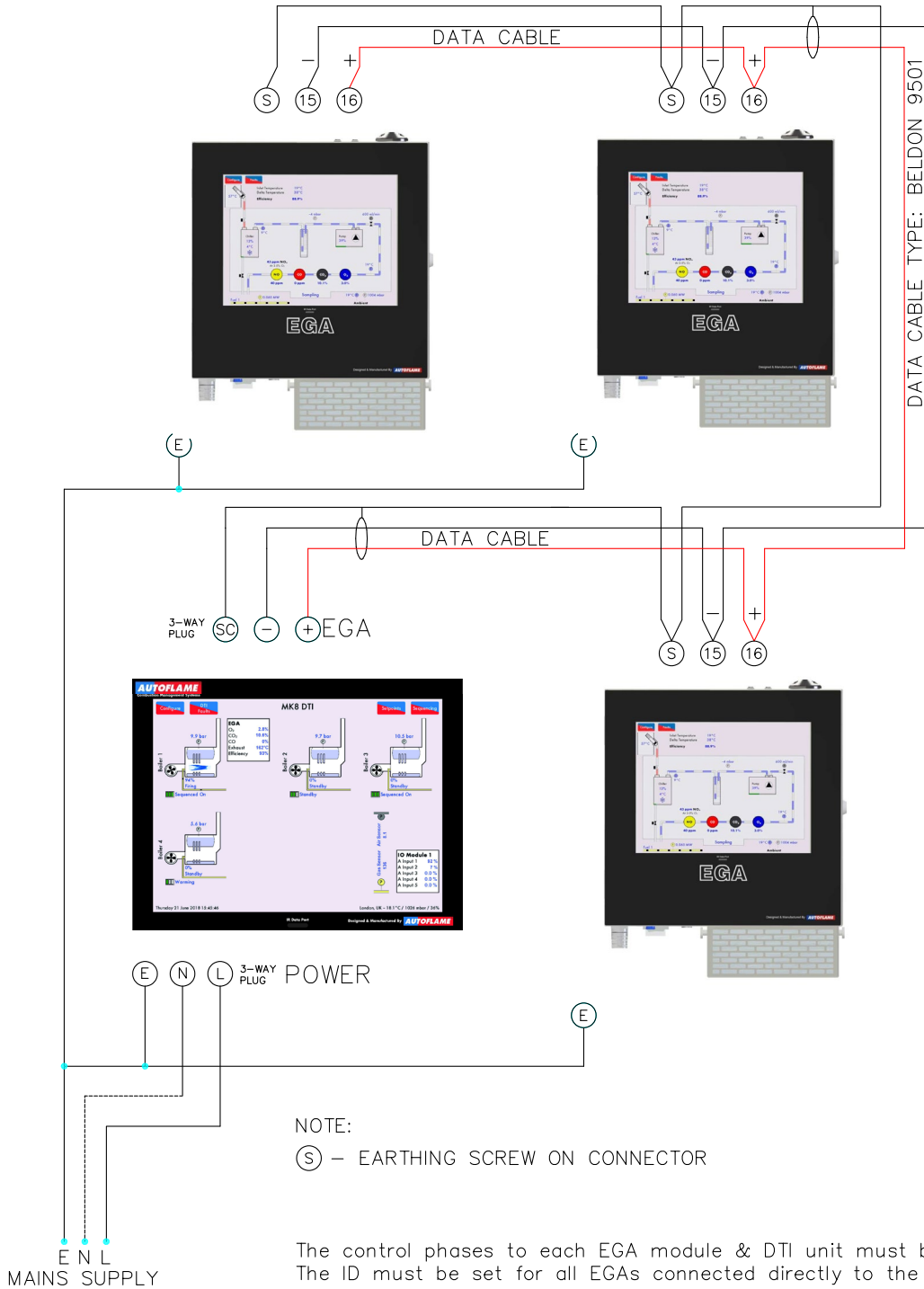
INTERCONNECTION BETWEEN STANDALONE E.G.A. MODULES AND D.T.I. MODULE
