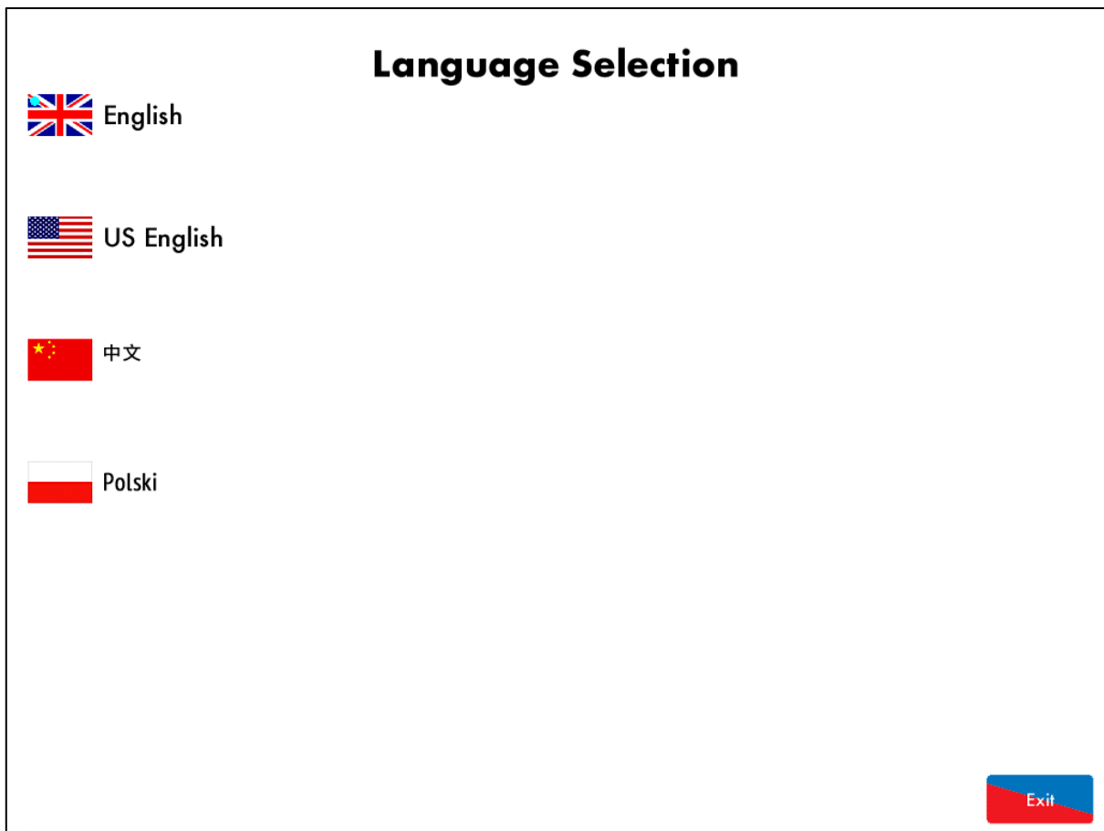
Figure 3.1.i Language Selection
